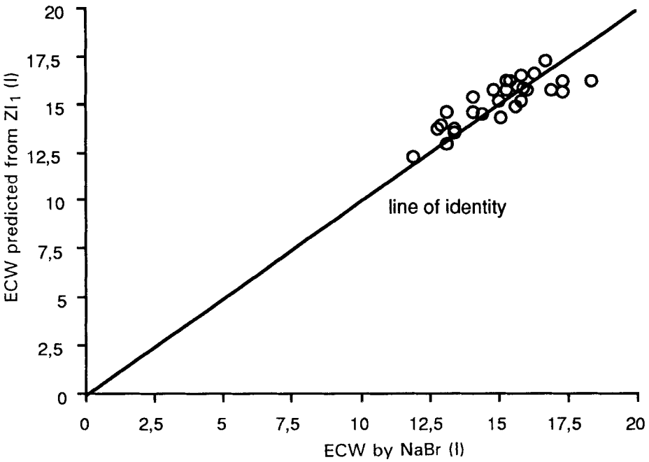
Figure 2. ECW estimated from height^2/Z_1 ( ZI_1 ; Deurenberg et al. 1993) against ECW obtained from NaBr dilution ( r=0.847 ).
