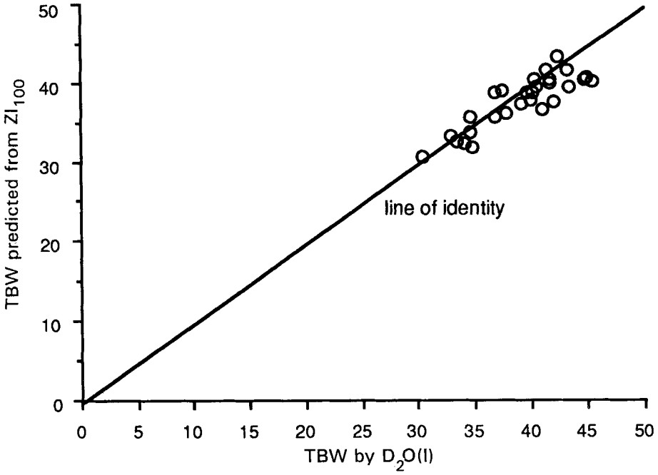
Figure 1. TBW predicted from height^2/Z_{100} ( ZI_{100} ; Deurenberg et al. 1993) against TBW obtained from D_2O dilution ( r=0.894 ).
